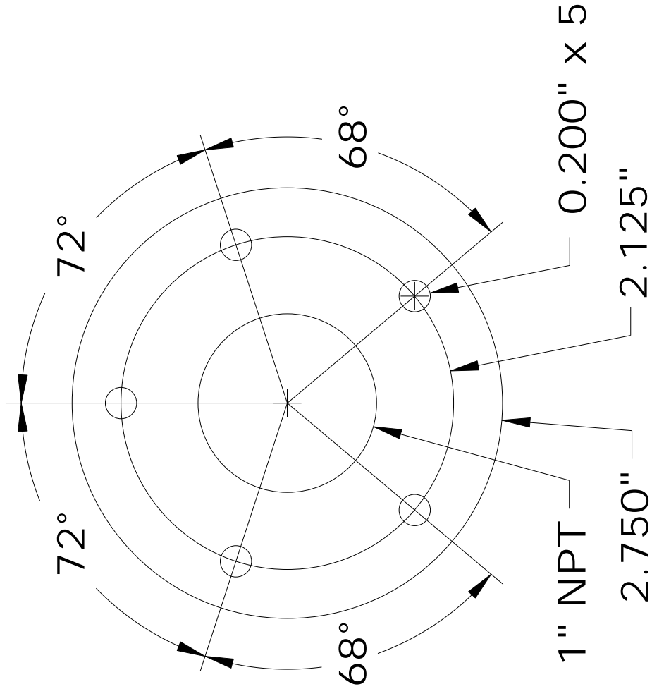
Figure 1: Mech. DWG of SAE-5 to 1" NPT Adapter.
